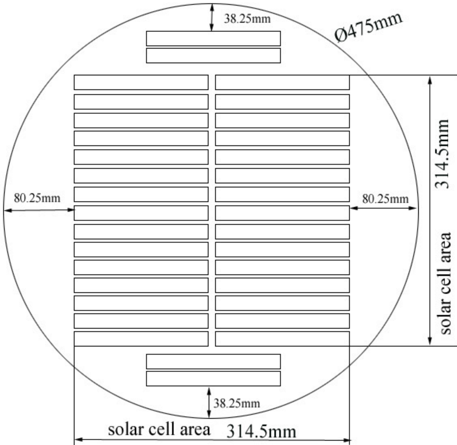
FRONT VIEW
