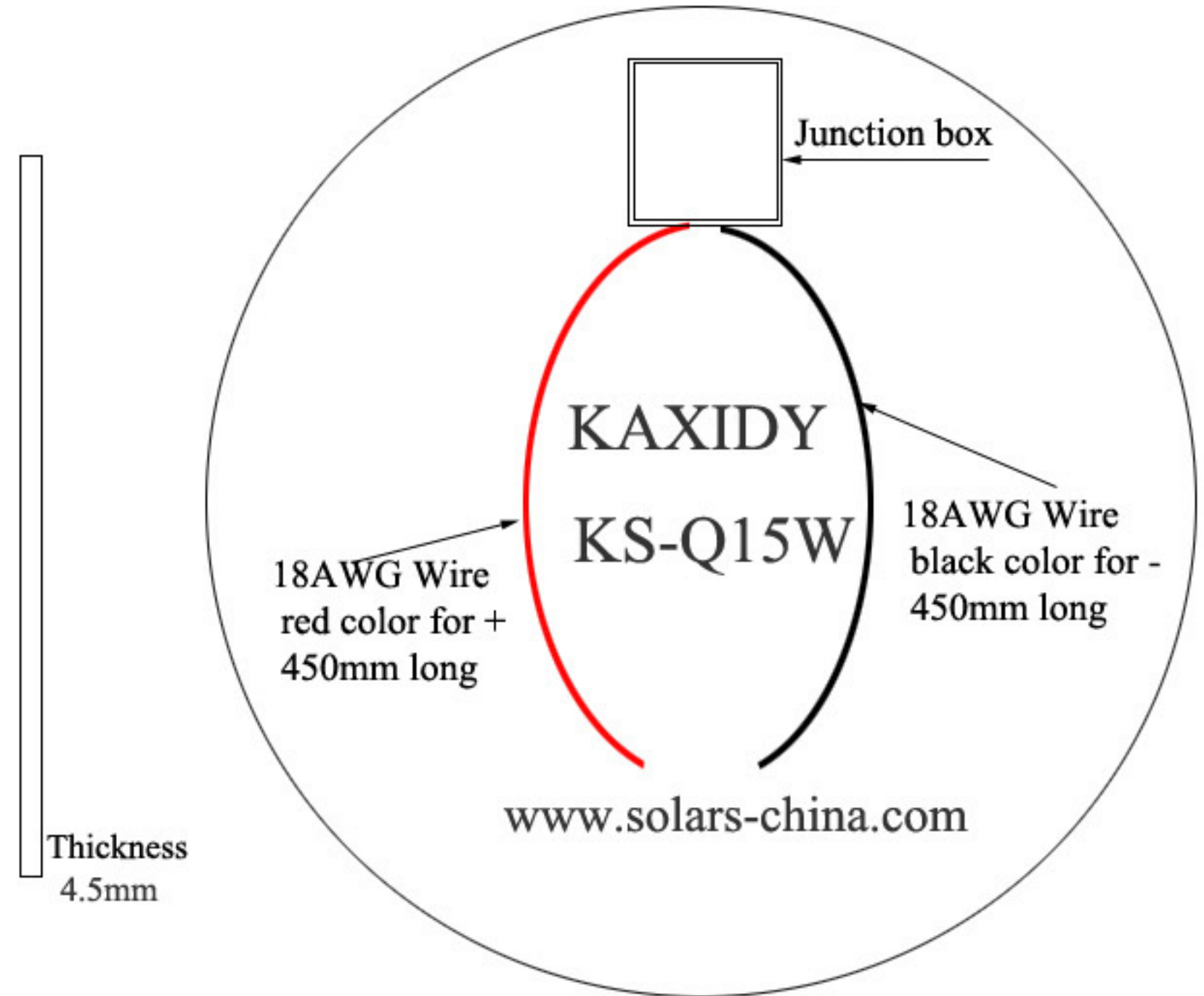
SIDE VIEW
