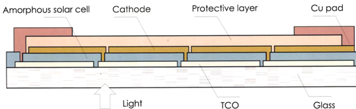
Structure of Amorphous Solar Cell
