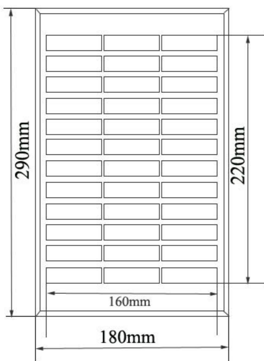
FRONT VIEW
