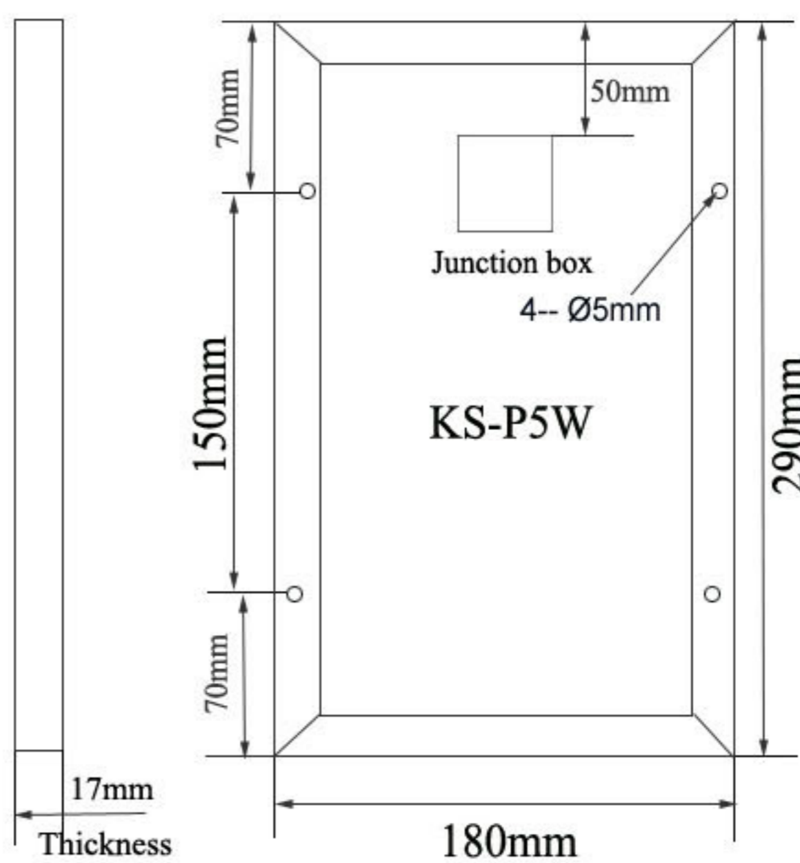
SIDE VIEW
